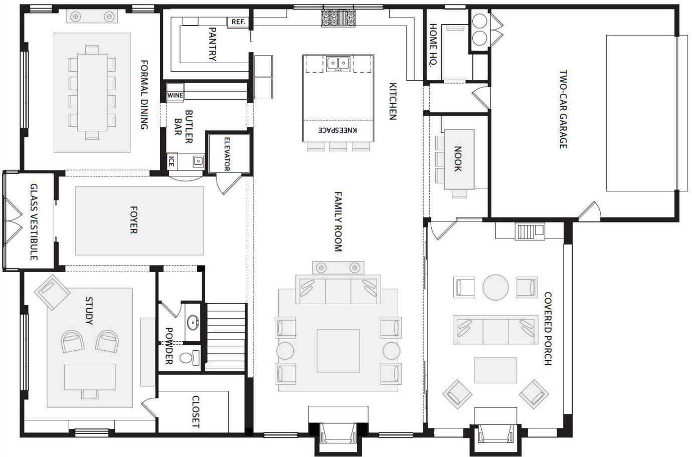
FIRST FLOOR
